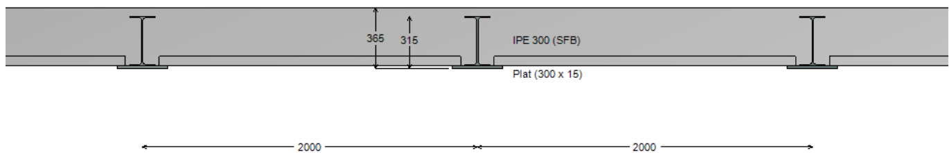
Figure 26 : Transversal view
