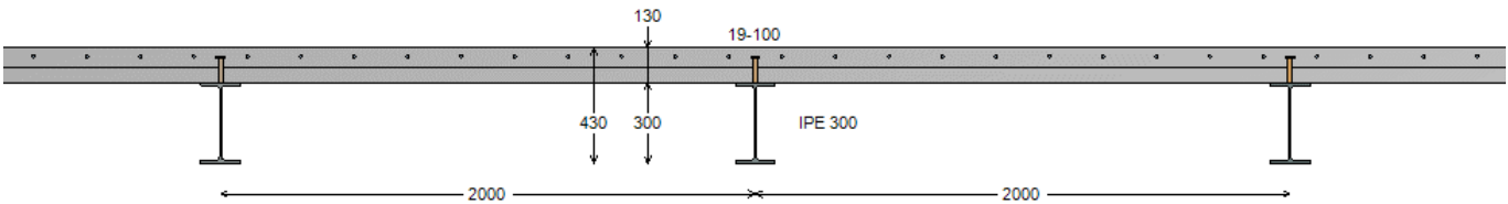
Figure 19 : Transversal view
