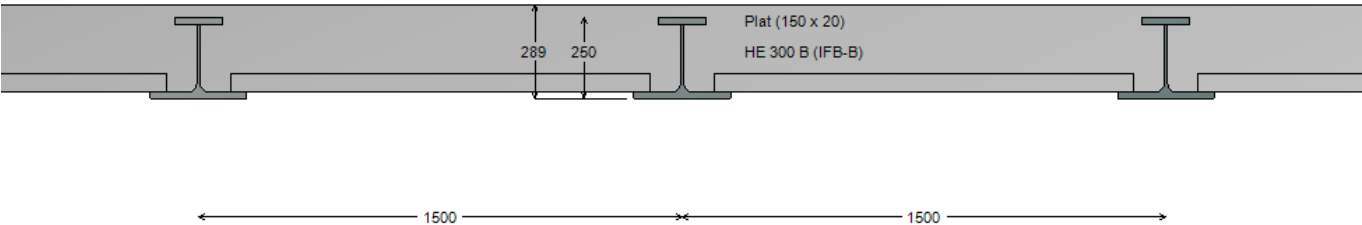
Figure 29 : Transversal view
