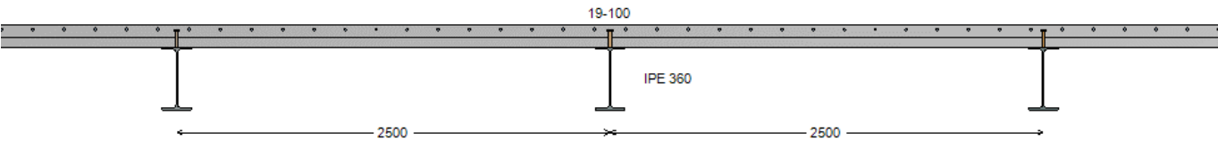
Figure 5 : Transversal view
