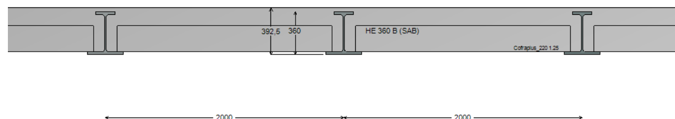
Figure 30 : Transversal view
