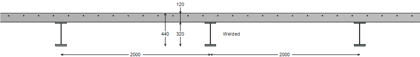
Figure 11 : Transversal view
