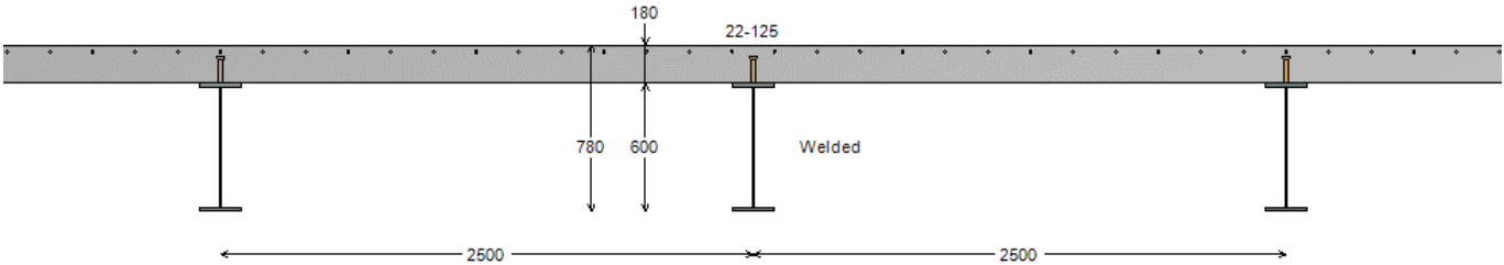
Figure 23 : Transversal view
