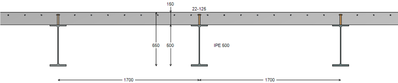
Figure 7 : Transversal view
