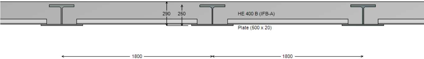
Figure 28 : Transversal view
