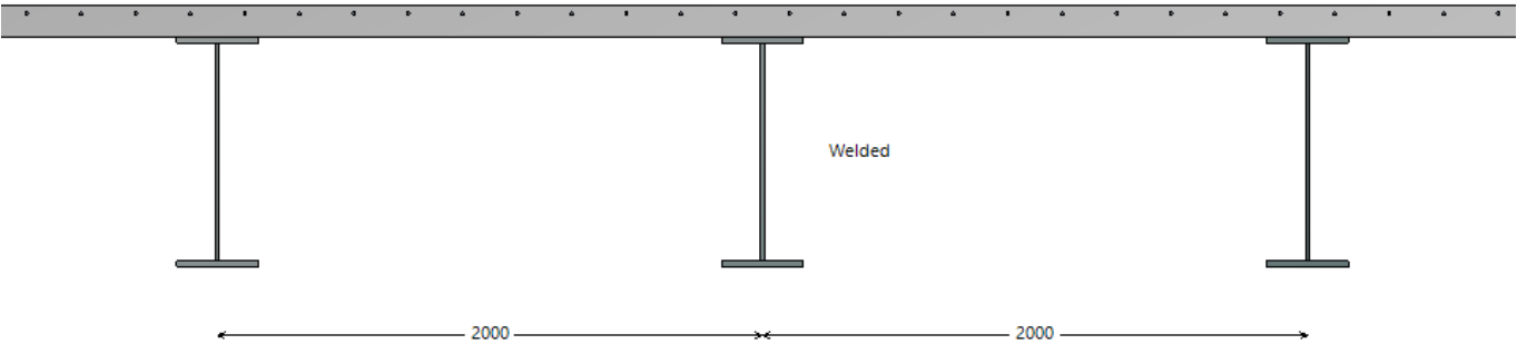
Figure 13 : Transversal view
